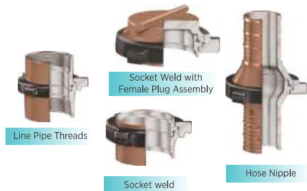
Suction Hose Unions - 500 PSI (34 bar) Maximum Line Pressure, 4", 5" & 6" sizes
