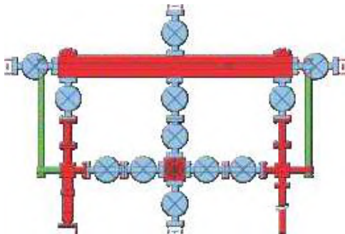
Choke Manifold
