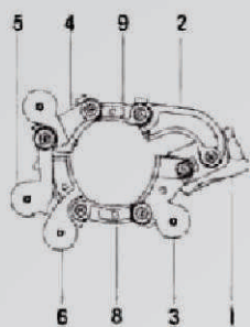
Fig A, 13.3/8"-14 1/2"
