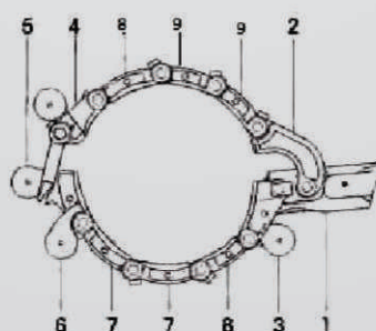
Fig K, 28.1/2"-30"
